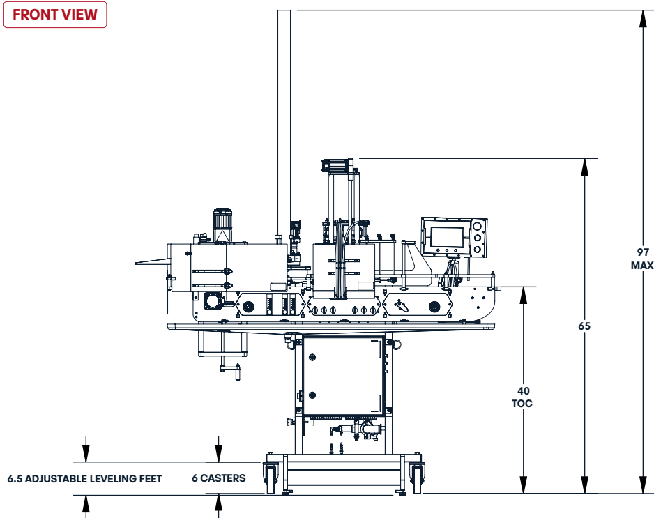
FRONT VIEW
